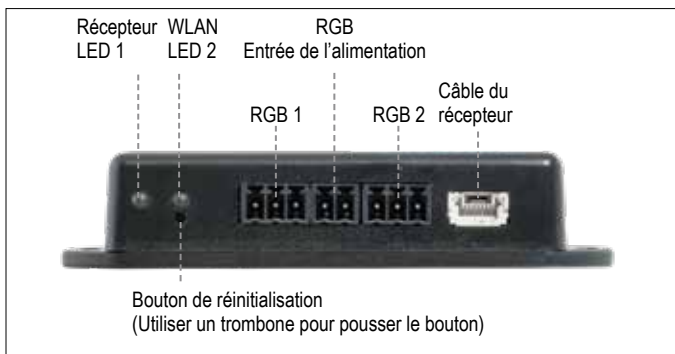
Figure 4: Wi-Fi Box (B6R-W2...)
