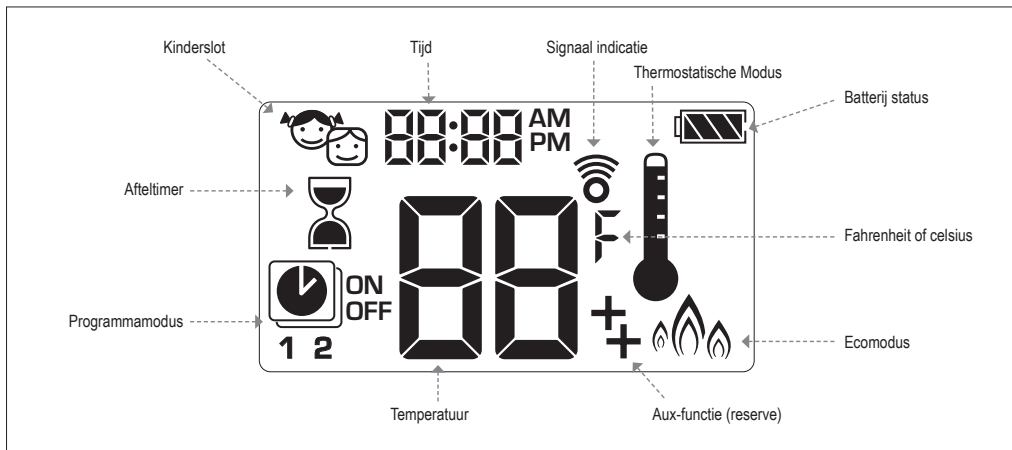
Afb. 21: 8-symbol Display
