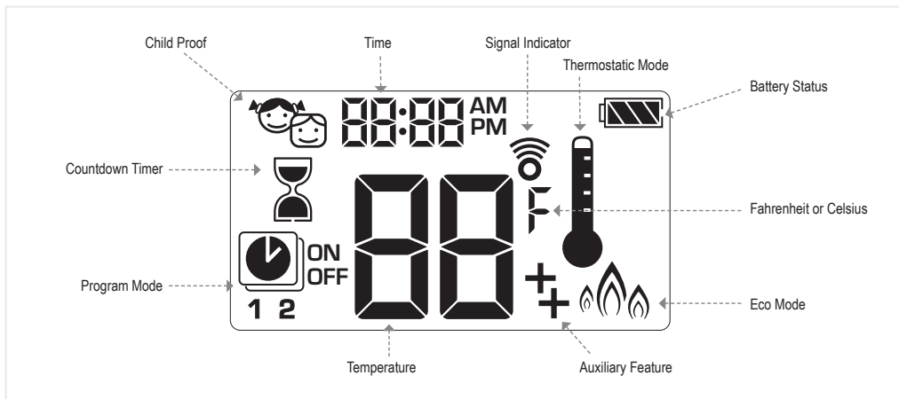
Figure 21: 8-symbol Display
