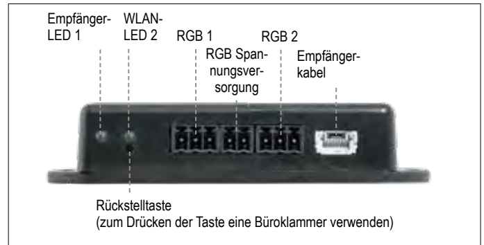
Abb. 3: Wi-Fi Box (B6R-W2...)
